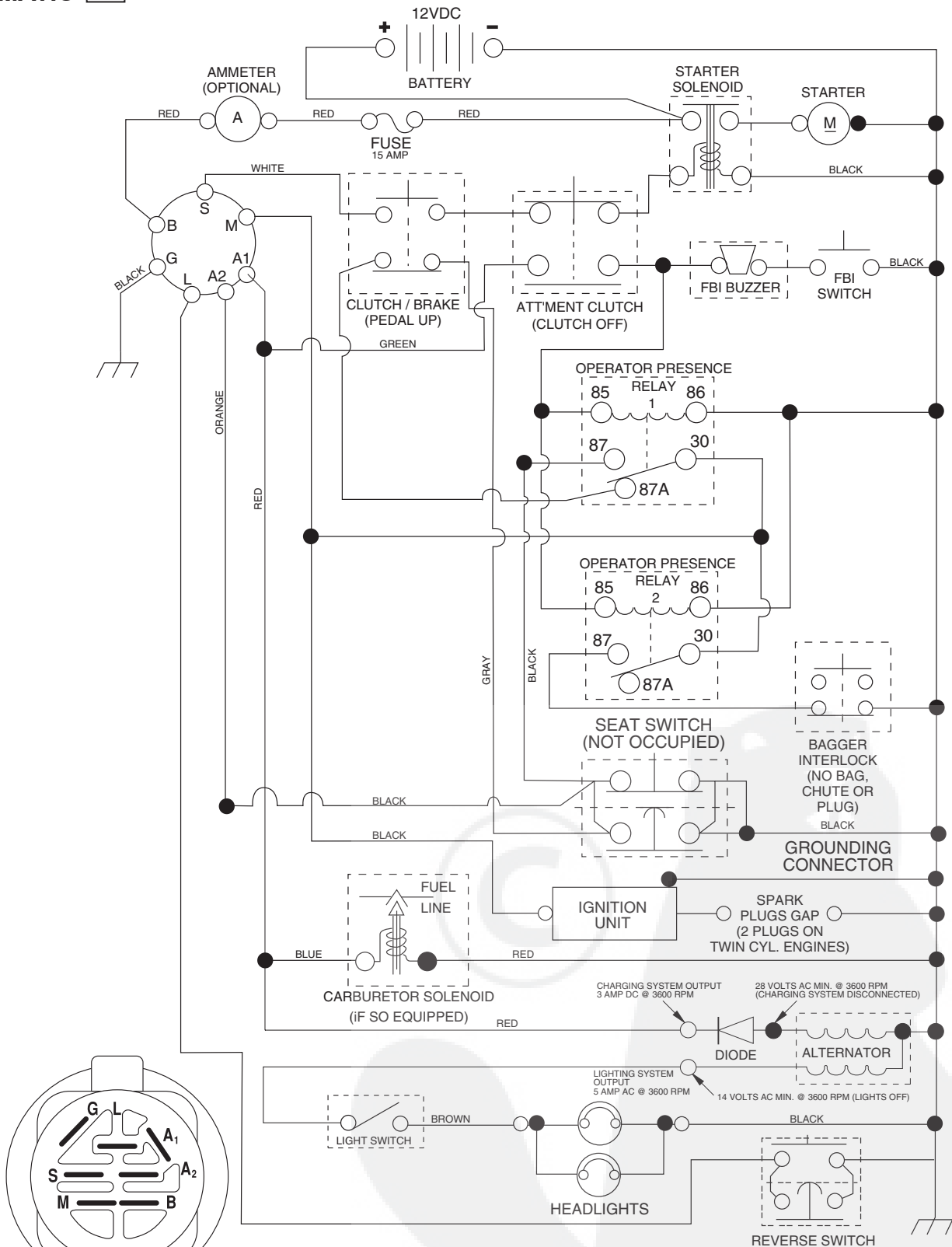
IGNITION SWITCH
