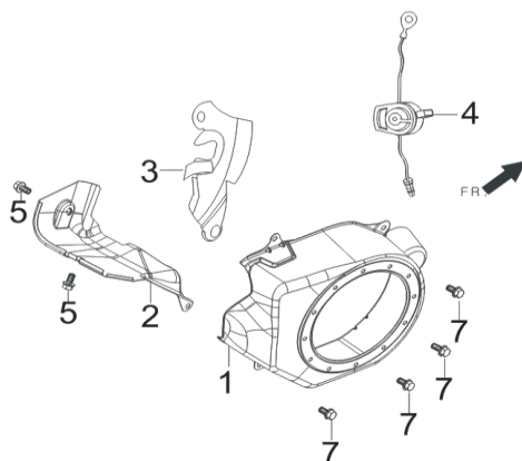
FIG.8 SHROUD / SHIELD,LOWER (E14)
