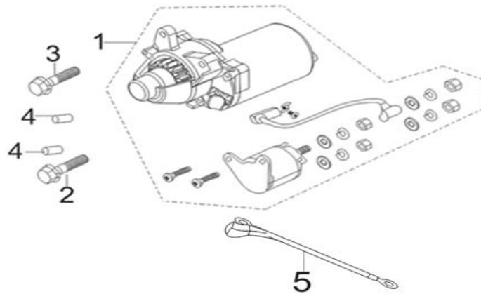
FIG.15 START-UP ELECTRIC MACHINE COMPONENTS (E09)
