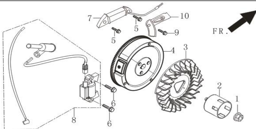
FIG.13 FLYWHEEL / IMPELLER / STARTER PULLEY / IGNITION COIL (E15)
