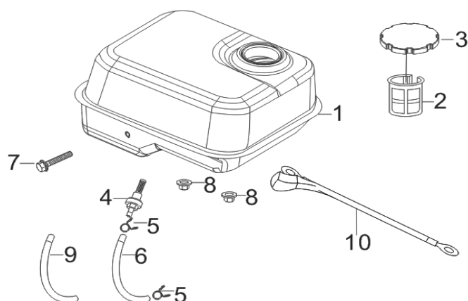
FIG.12 TANK ASSY, FUEL (F01)
