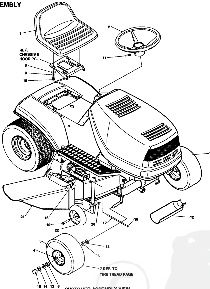
CUSTOMER ASSEMBLY VIEW 322770 PARTS BAG ASSY QTY1
