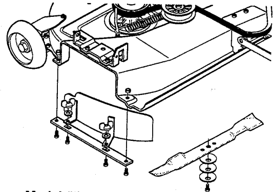
Model #5715-00 Mulching Kit (39" Deck)
