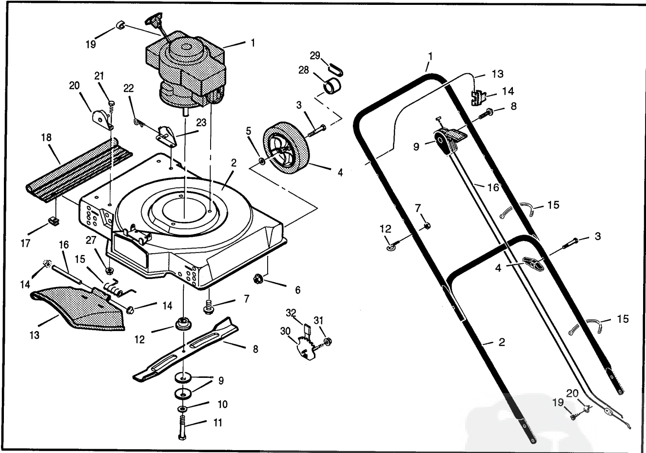
MOWER HOUSING PARTS LIST
