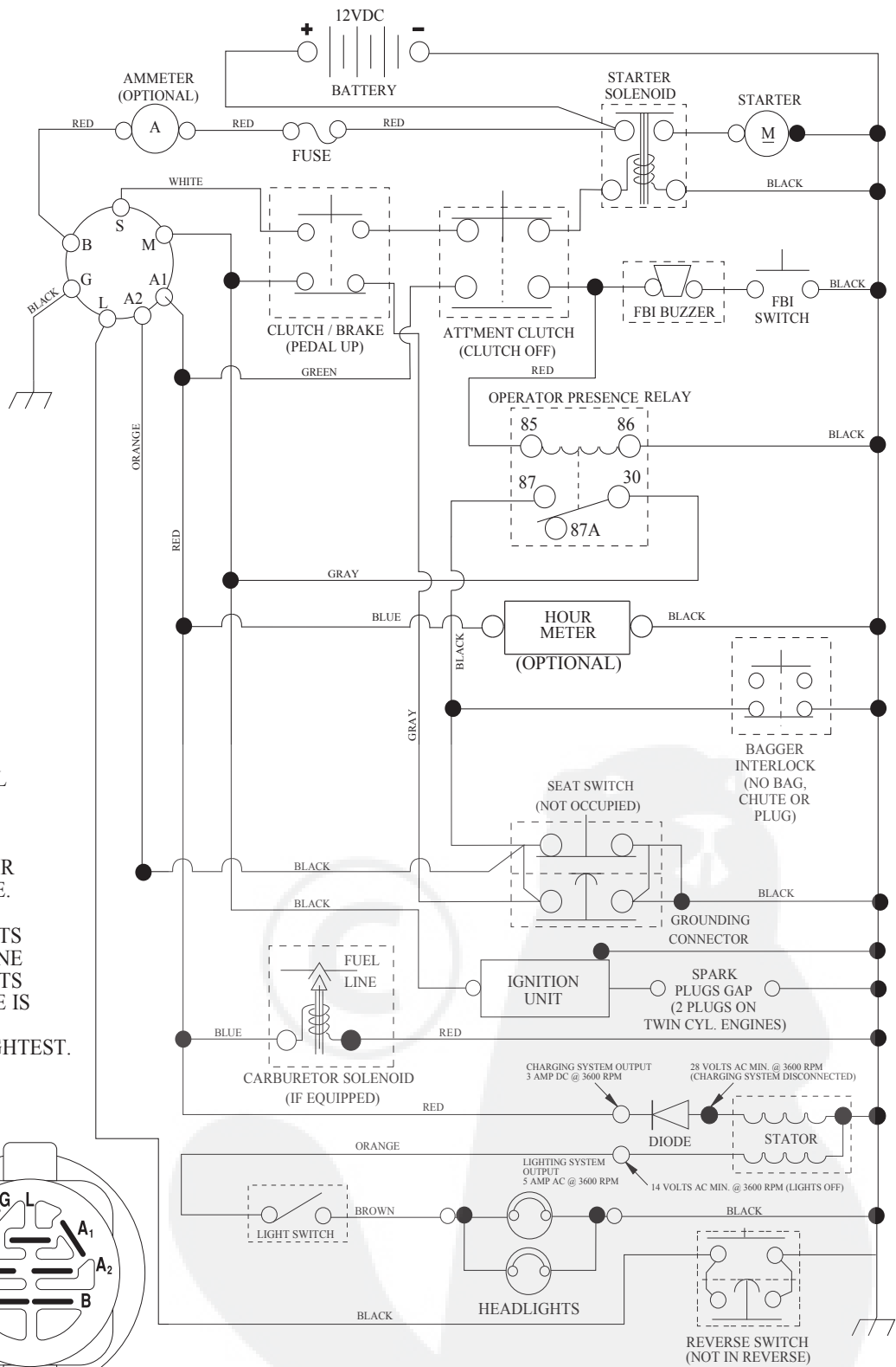
IGNITION SWITCH
