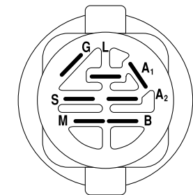
IGNITION SWITCH
