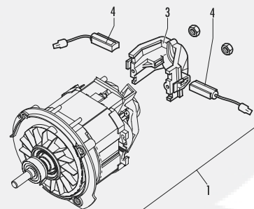
FIGURE 3 - 1850 W
