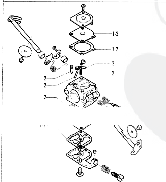
FIGURE 3 - CARB. ZAMA C1Q-EL1
