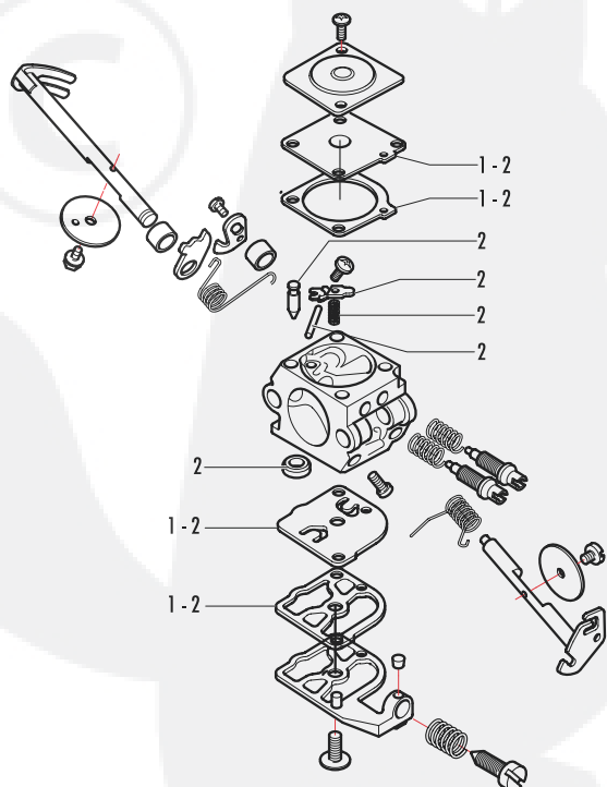
FIGURE 3 - WALBRO WT 170
