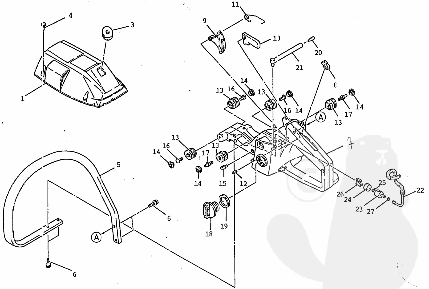
3. HANDLE
